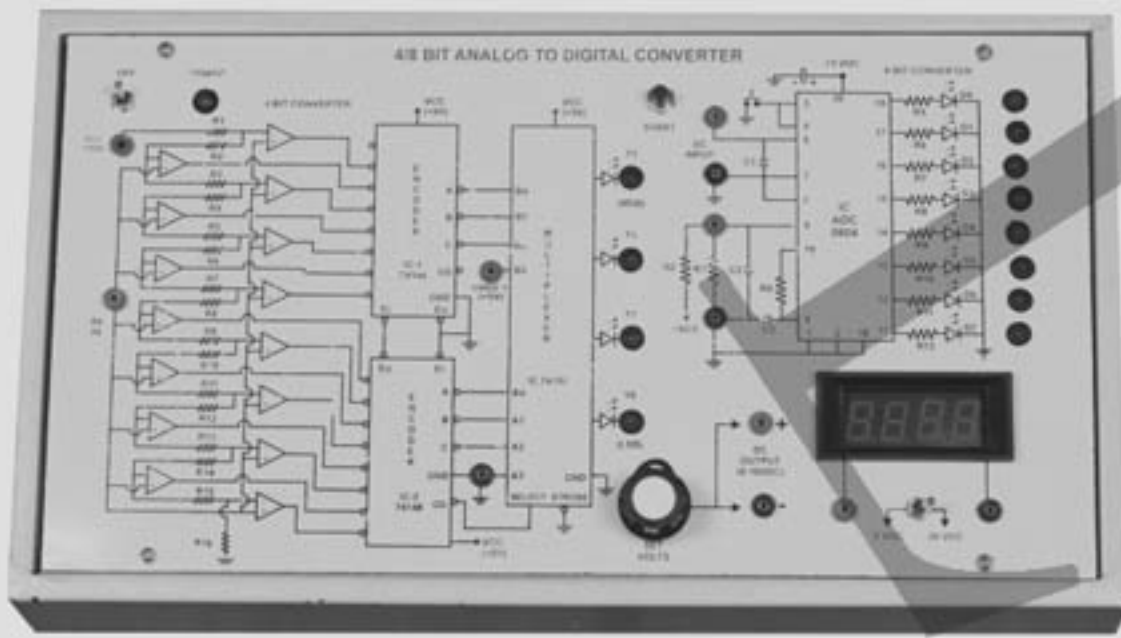
4/8 Bit Analog to Digital Converter
