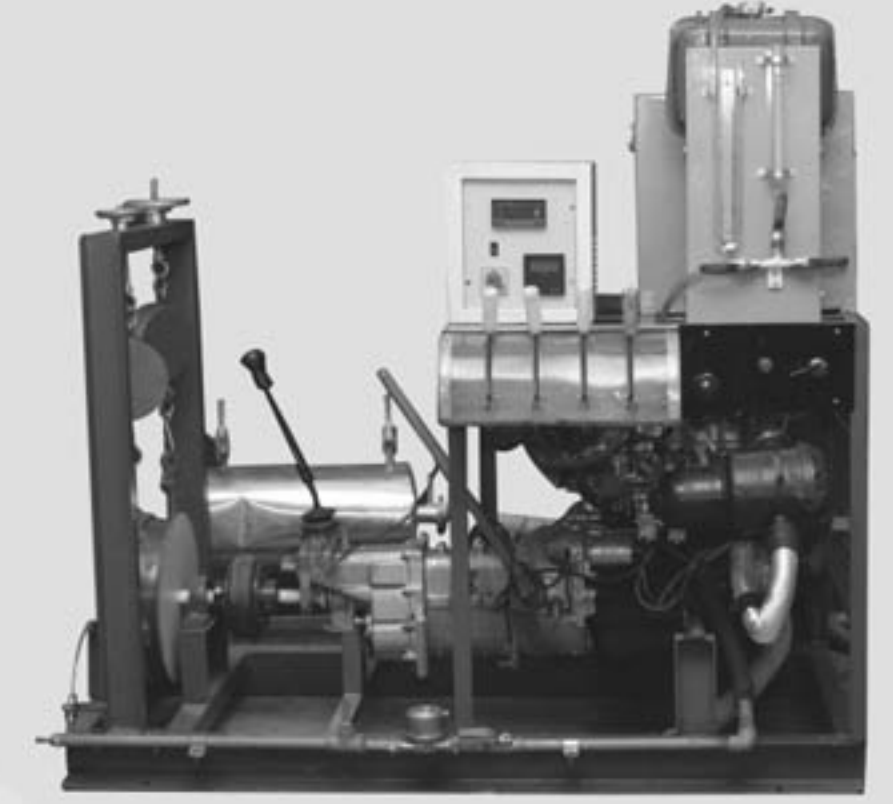
Petrol Engine Test Rig
