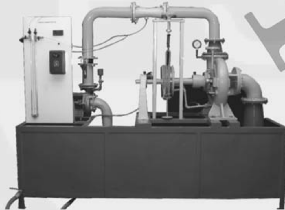
Francis Turbine
